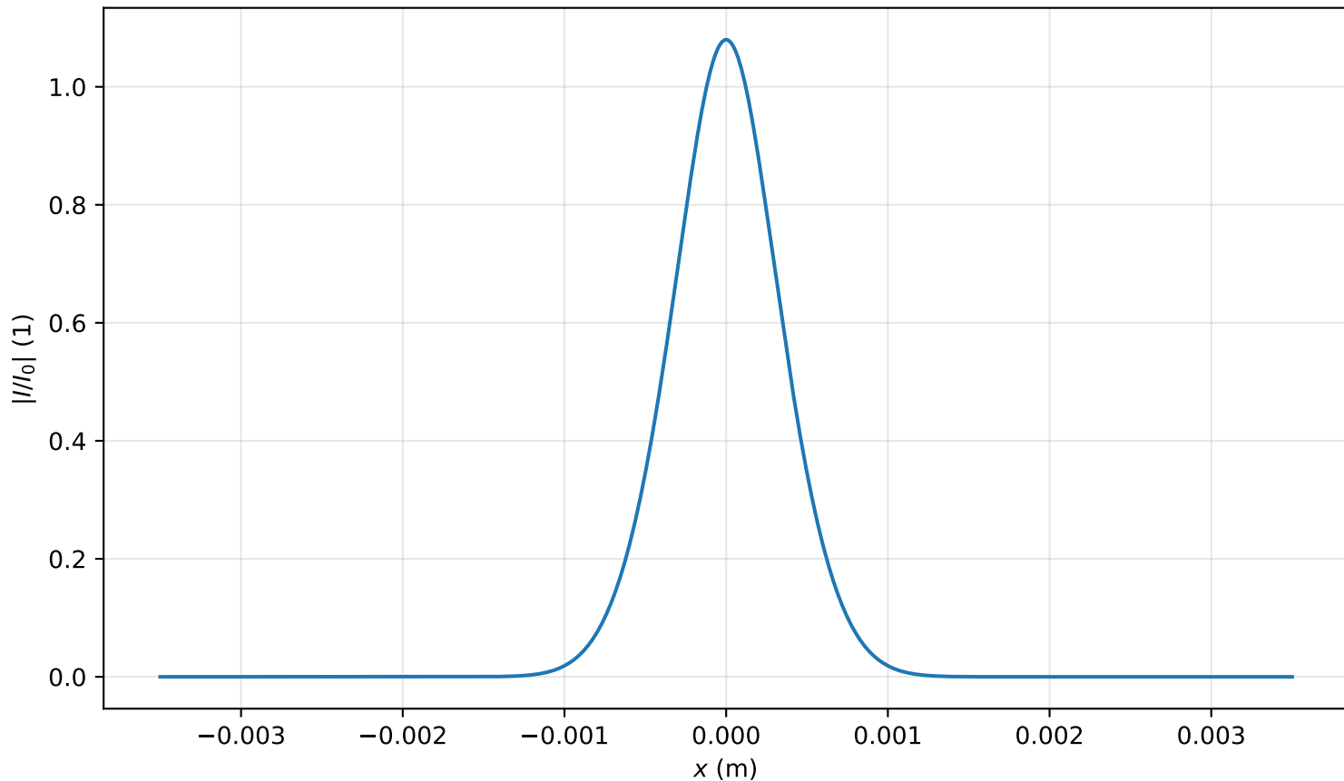
Intensity profile I(x, y = 0, z = 0.398m)/I_0 , P_{in}=0.8P_{cr} , artificial time
